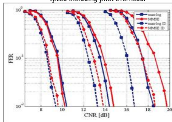
Figure 9. FER vs. CNR of iterative decoding with 8 bps and code rates 1/3, 8/15 and 11/15 in the NGH Outdoor MIMO channel with 60 km/h speed.
