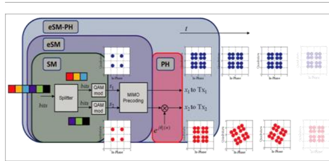
Figure 6. Diagram multiplexing techniques: SM (Spatial Multiplexing), eSM (enhanced Spatial Multiplexing) and PH (Phase Hopping), and the combination of them, eSM-PH (enhanced-Spatial Multiplexing – Phase Hopping).
