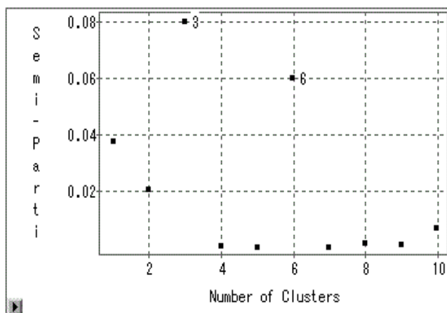
FIGURE 4-5 R^2 STATISTICS
