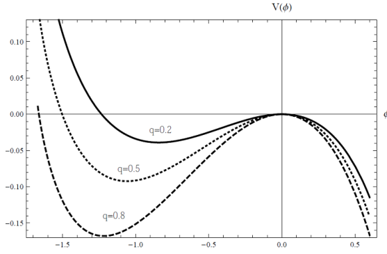
FIGURE 3. VARIATION OF SAGDEEV POTENTIAL V(\phi) with \phi for range 0 < q < 1 with \beta = 1 , \sigma = 0.01 and M = 2 .
