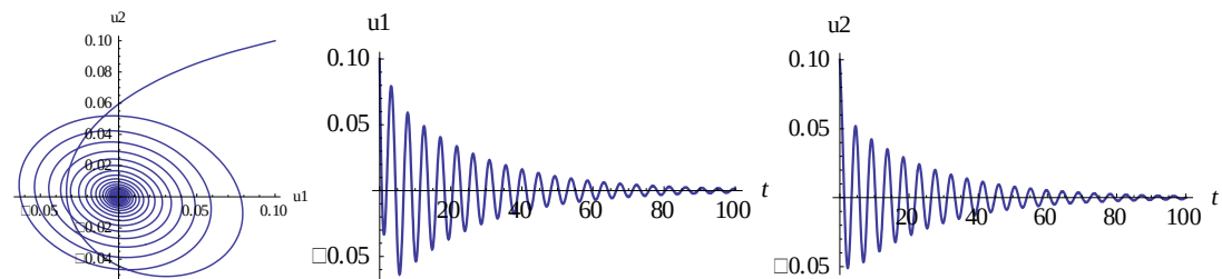
FIGURE 7: THE EQUILIBRIUM E^* IS LOCALLY ASYMPTOTICALLY STABLE WITH \tau_1 = 0.1 < \tau_{1*}, \tau_2 = 1.2
