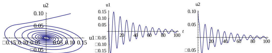
FIGURE 1: THE EQUILIBRIUM E^* IS LOCALLY ASYMPTOTICALLY STABLE WITH \tau_1 = 1.8 < \tau_{10}
