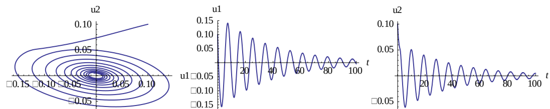
FIGURE 9: THE EQUILIBRIUM E^* IS LOCALLY ASYMPTOTICALLY STABLE WITH \tau_1 = 1.8, \tau_2 = 0.2 < \tau_2^*
