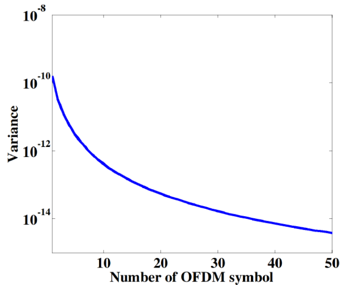
FIGURE 12: VARIANCE OF THE ESTIMATOR ACCORDING TO THE NUMBER OF SYMBOL M.
