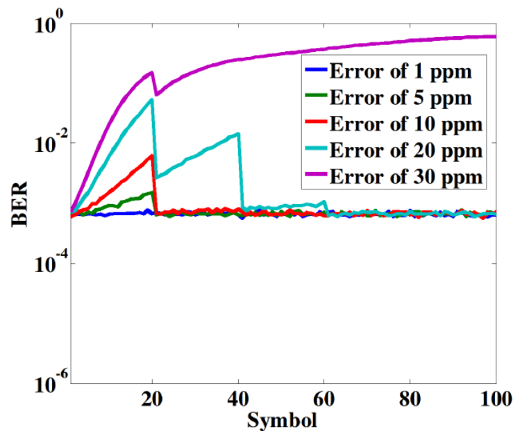
FIGURE 13: BER ACCORDING TO THE NUMBER OF OFDM SYMBOL.
