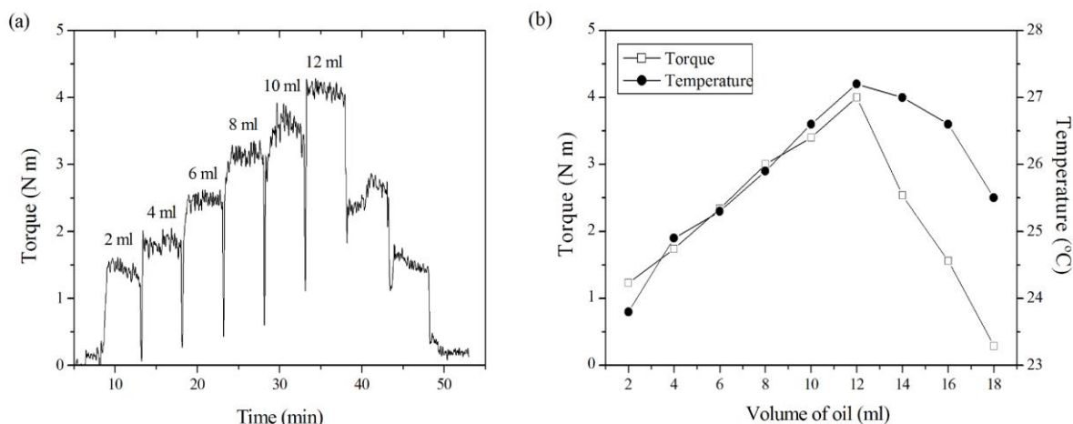
FIGURE 5. (A) TORQUE VARIATION WITH MIXING TIME FOR DIFFERENT ADDITIONS OF OIL; (B) TORQUE AND TEMPERATURE VALUES FOR DIFFERENT OIL VOLUMES.
