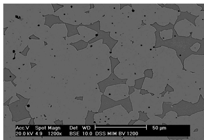
FIGURE 9. MICROSTRUCTURE OF INJECTION-MOULDED DUPLEX STAINLESS STEEL SINTERED AT 1250 °C.
