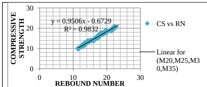
FIG 1. LINEAR RELATION BETWEEN COMPRESSIVE STRENGTH & REBOUND NUMBER
