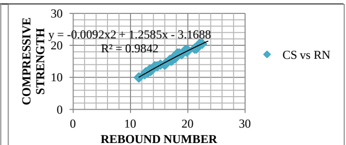
FIG 2. QUADRATIC RELATION BETWEEN COMPRESSIVE STRENGTH & REBOUND NUMBER
