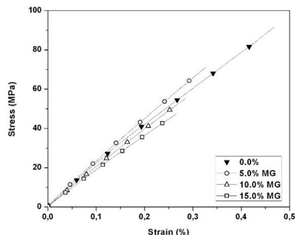
FIGURE 4: Stress X strain curves for different fractions of micronized graphite (MG) and material without conductive fillers.
