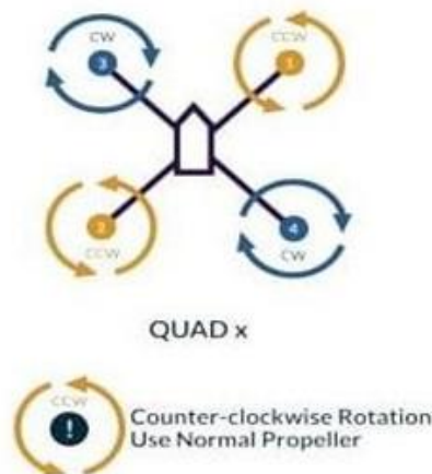
FIGURE 1: Propeller configuration of quadcopter
