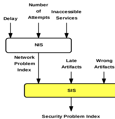
FIG.3. FUZZY INFERENCE SYSTEMS FOR INTRUSION DETECTION IN THE CLOUD
