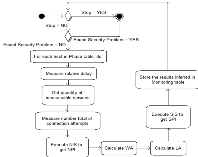
FIG.4. THE SOFTMANCLOUD'S MONITORING ALGORITHM
