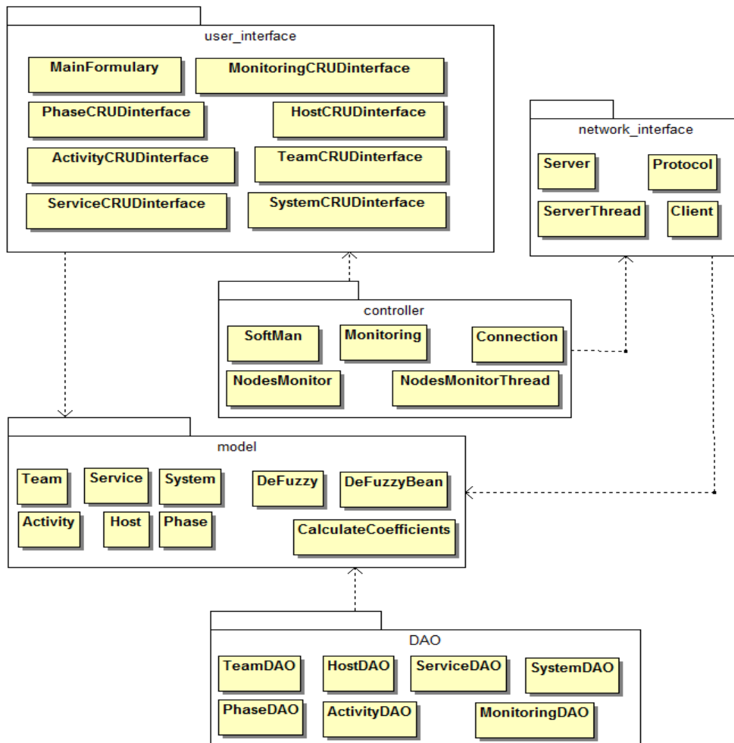
FIG.2. THE SOFTMANCLOUD PROGRAM CLASS MODEL
