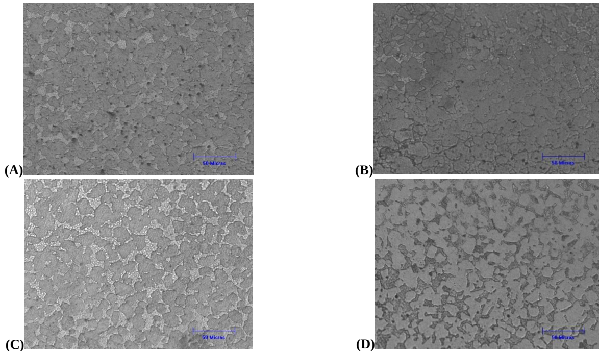
FIGURE 8: COMPARISON OF THE TEST TUBES OF BRASS 60-40 ATTACKED WITH 2G K 2 Cr 2 O 7 + 8mLH 2 UNDER4+ 4DROOP HCL+100mL TOILET ACCORDING TO THE NORM ASTM AND-407 MAY 2011 DURING 10 SECONDS. (A) TEST TUBE OF BRASS 60-40 SUBJECTED TO 24 HOURS OF CRYOGENIC TREATMENT. (B) TEST TUBE OF BRASS 60-40 SUBJECTED TO 48 HOURS OF CRYOGENIC TREATMENT. (C) TEST TUBE OF BRASS 60-40 SUBJECTED TO 72 HOURS OF CRYOGENIC TREATMENT. (D) TEST TUBE OF BRASS 60-40 SUBJECTED TO 120 HOURS OF CRYOGENIC TREATMENT. AUTHOR OF THE PROJECT 2016.
