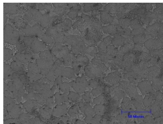
FIGURE 4 BRASS 60-40 500 X
