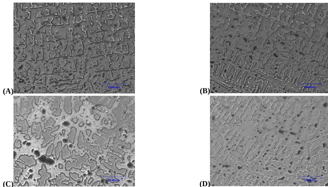
FIGURE 9: COMPARISONS OF THE TEST TUBES OF BRONZE SAE 64 ATTACKED WITH 2 g FeCl 3 + 5 mLHCl+ 30 mL toilet + 60 mL ETHANOL OR METHANOL ACCORDING TO THE NORM ASTM E-407 MAY 2011. (A) TEST TUBE OF BRONZE SAE 64 SUBJECTED TO 24 HOURS OF CRYOGENIC TREATMENT. (B) TEST TUBE OF BRONZE SAE 64 SUBJECTED TO 48 HOURS OF CRYOGENIC TREATMENT. (C) TEST TUBE OF BRONZE SAE 64 SUBJECTED TO 72 HOURS OF CRYOGENIC TREATMENT. (D) TEST TUBE OF BRONZE SAE 64 SUBJECTED TO 120 HOURS OF CRYOGENIC TREATMENT. AUTHOR OF THE PROJECT 2016
