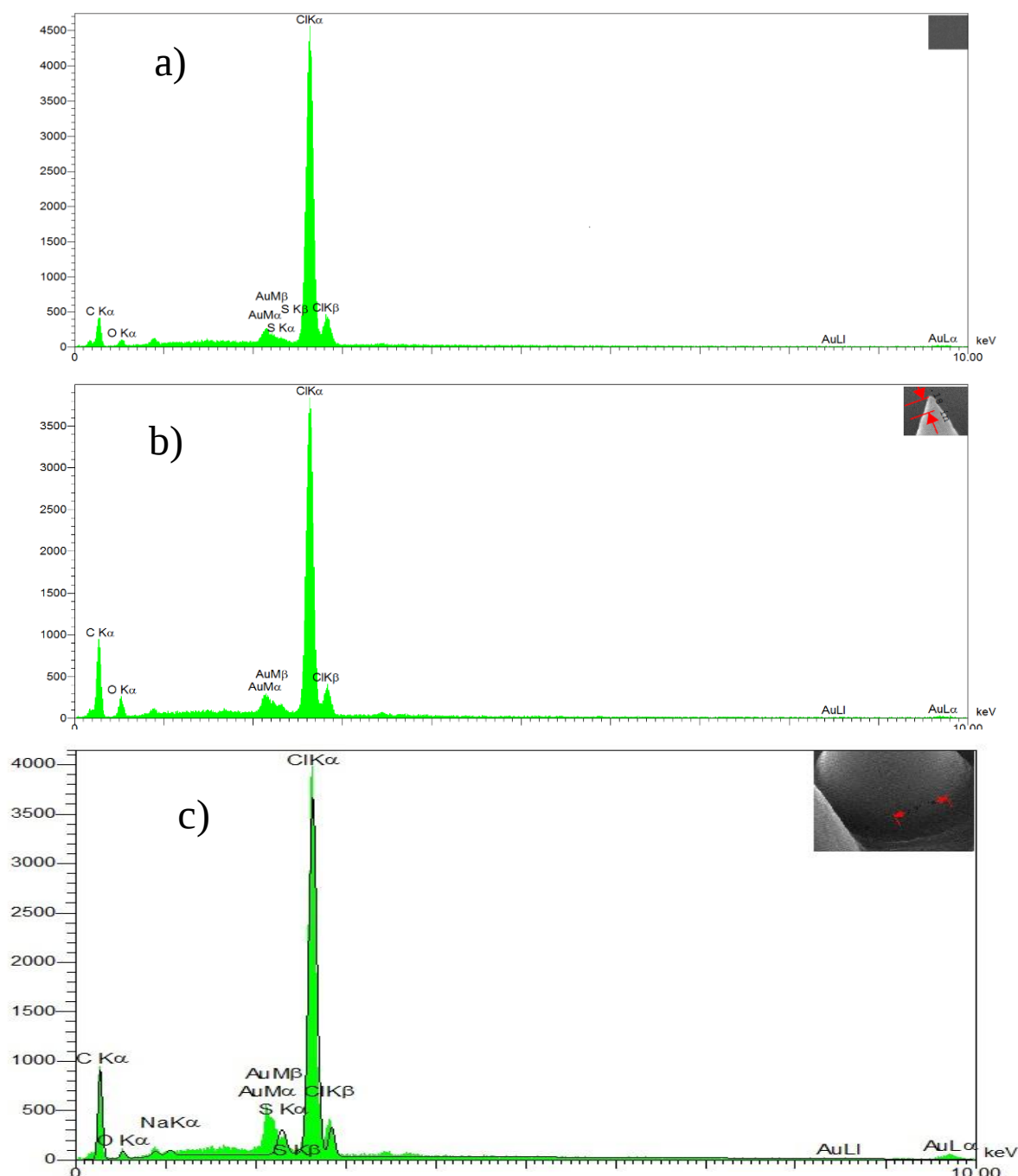
FIGURE 2. THE CREATED EDX SPECTRA OF CONES ON PET POLYMERS.
