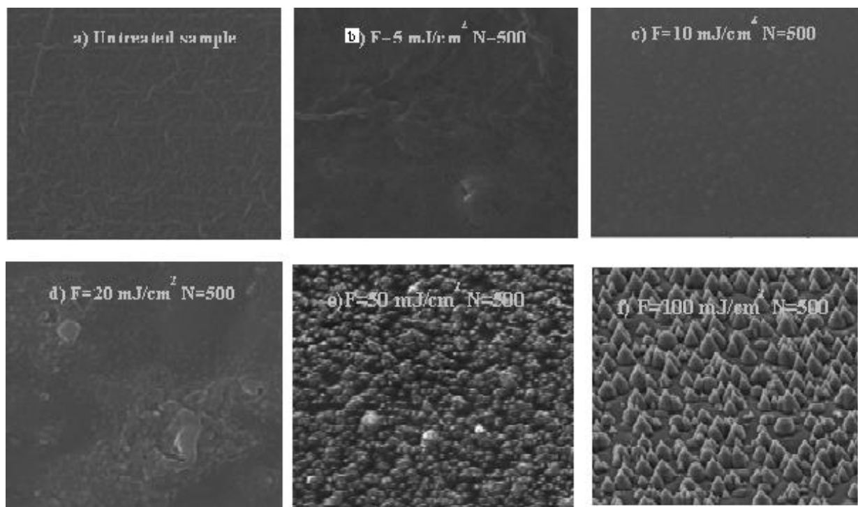
FIGURE 1. SEM OF ABLATED AREA IN PET POLYMER WITH CONSTANT NUMBER OF PULSES (N=500) AND DIFFERENT FLUENCES A) UNTREATED SAMPLE, B) 5\text{ mJ/cm}^2 , c) 10\text{ mJ/cm}^2 , d) 20\text{ mJ/cm}^2 , e) 50\text{ mJ/cm}^2 and f) 100\text{ mJ/cm}^2 .
