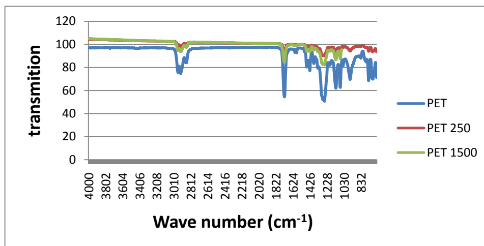
FIGURE 3. FTIR SPECTRUM OF UNTREATED AND IRRADIATION SAMPLE OF A PET POLYMER AT 50 mJ/cm 2 with 250 and 1500 pulses.
