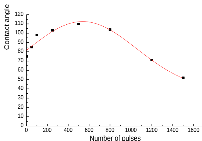
FIGURE 4. THE CONTACT ANGLE OF WATER VERSUS THE NUMBER OF LASER PULSES FOR PET POLYMER AT THE FLUENCE OF 50 mJ/cm 2 .
