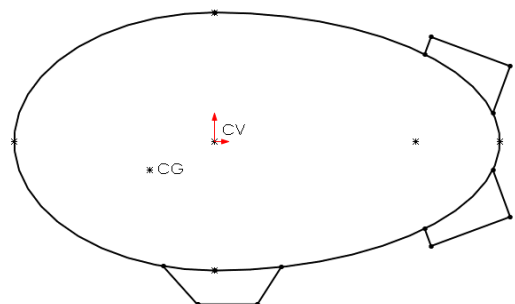
FIGURE 3. CENTER OF GRAVITY AND CENTER OF VOLUME OF A DIRIGIBLE.
