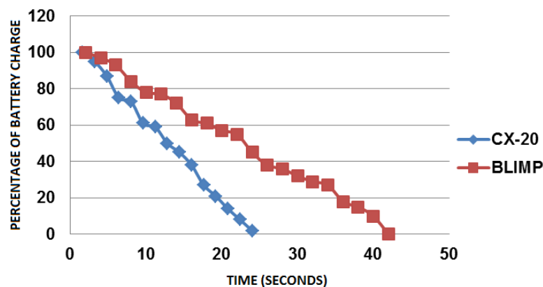
FIGURE 14. AUTONOMY DIRIGIBLE VS DRONE
