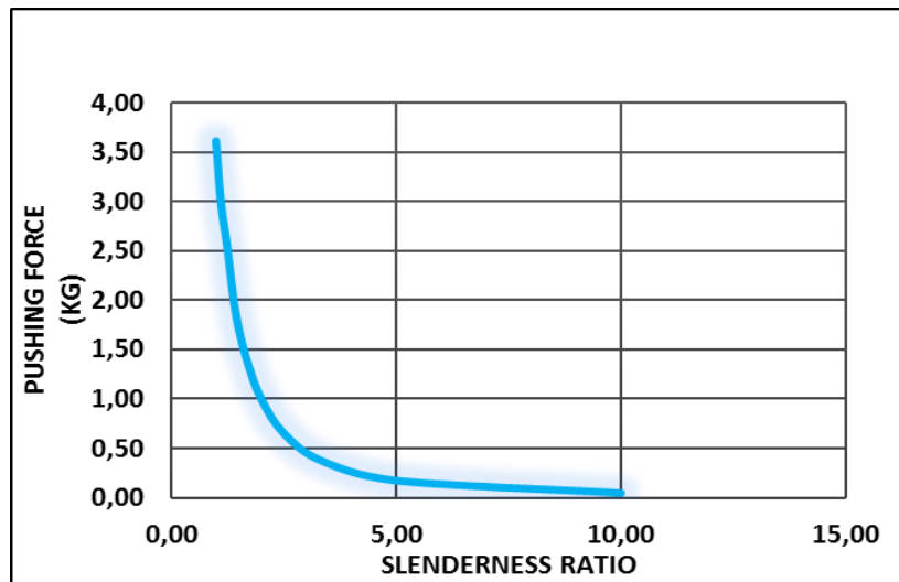
FIGURE 1. SLENDERNESS RATIO VS. PUSHING FORCE
