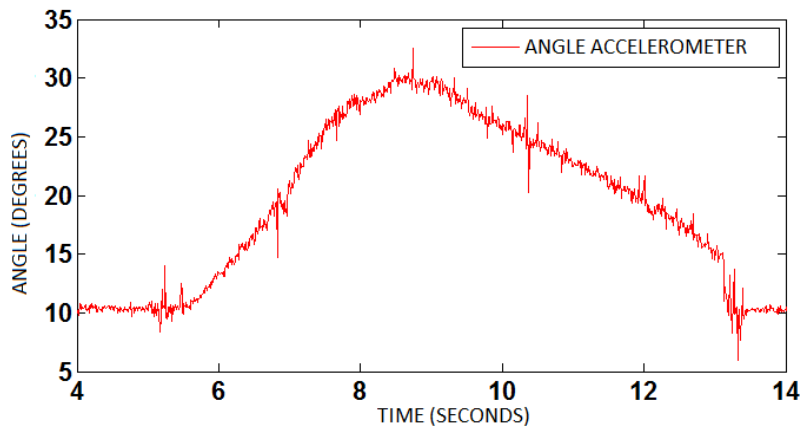
FIGURE 7 CALCULATION TILT ACCELEROMETER
