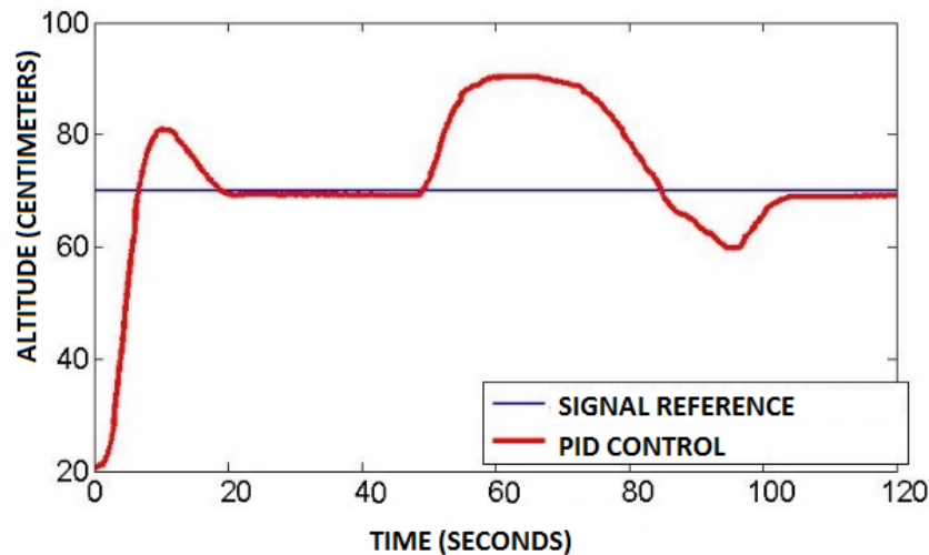
FIGURE 13 RESPONSE HEIGHT SYSTEM, CONTROLLED BY PID AFTER BEING DISTURBED
