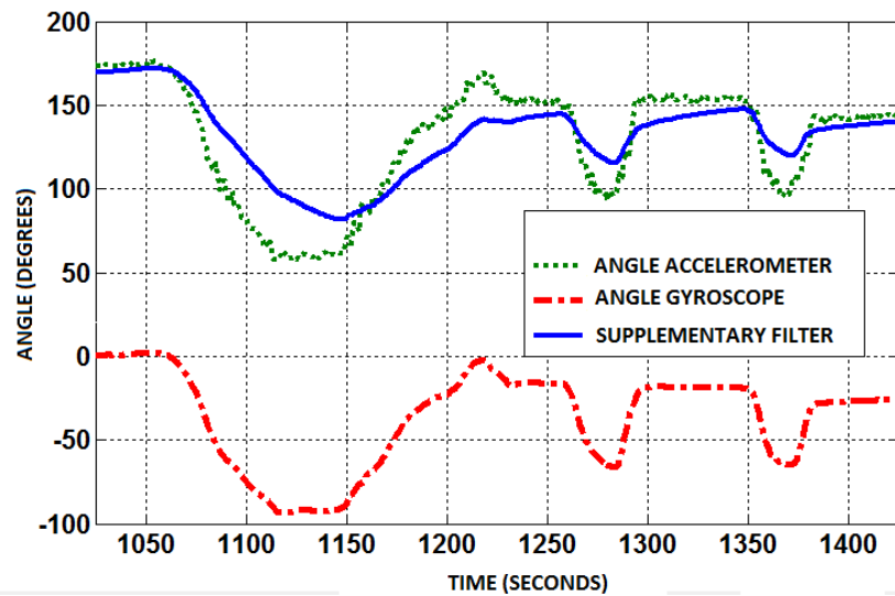
FIGURE 10 RESULT COMPLEMENTARY FILTER
