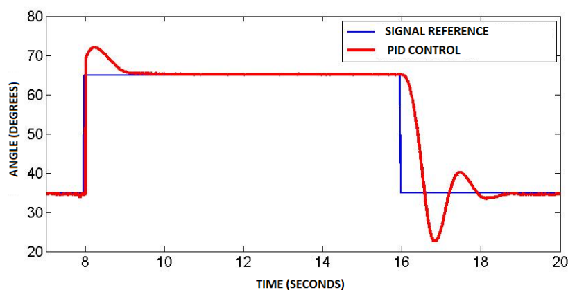
FIGURE 12. RESPONSE TURNING SYSTEM CONTROLLED BY PID ABOUT 30^\circ
