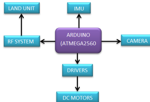
FIGURE 5 SYSTEM ARCHITECTURE
