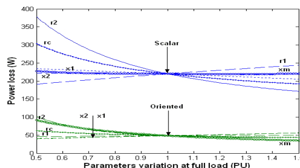
FIG. 33 VARIATION OF POWER LOSS WITH PARAMETERS AT 100 HZ
