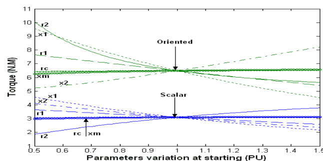
FIG. 8 VARIATION OF TORQUE WITH PARAMETERS AT 100 Hz
