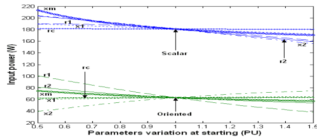
FIG. 12 VARIATION OF INPUT POWER WITH PARAMETERS AT 10 HZ
