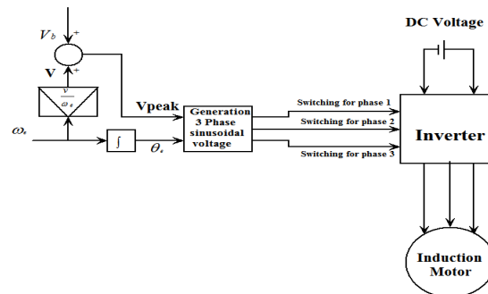
FIG. 2 OPEN LOOP SCALAR CONTROL
