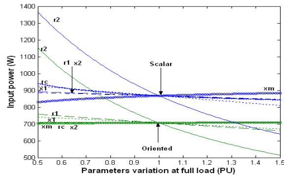
FIG. 27 VARIATION OF INPUT POWER WITH PARAMETERS AT 100 Hz
