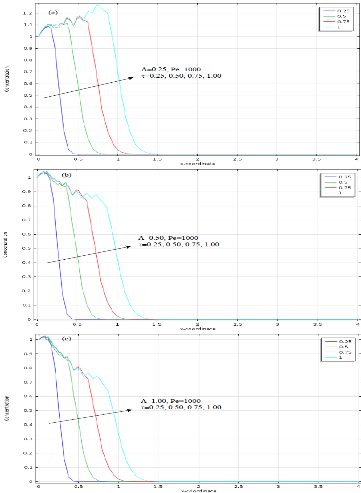
FIGURE 3: CONTINUOUS SOURCE LINE GRAPHS FOR CONCENTRATION VS. LONGITUDINAL DISTANCE
