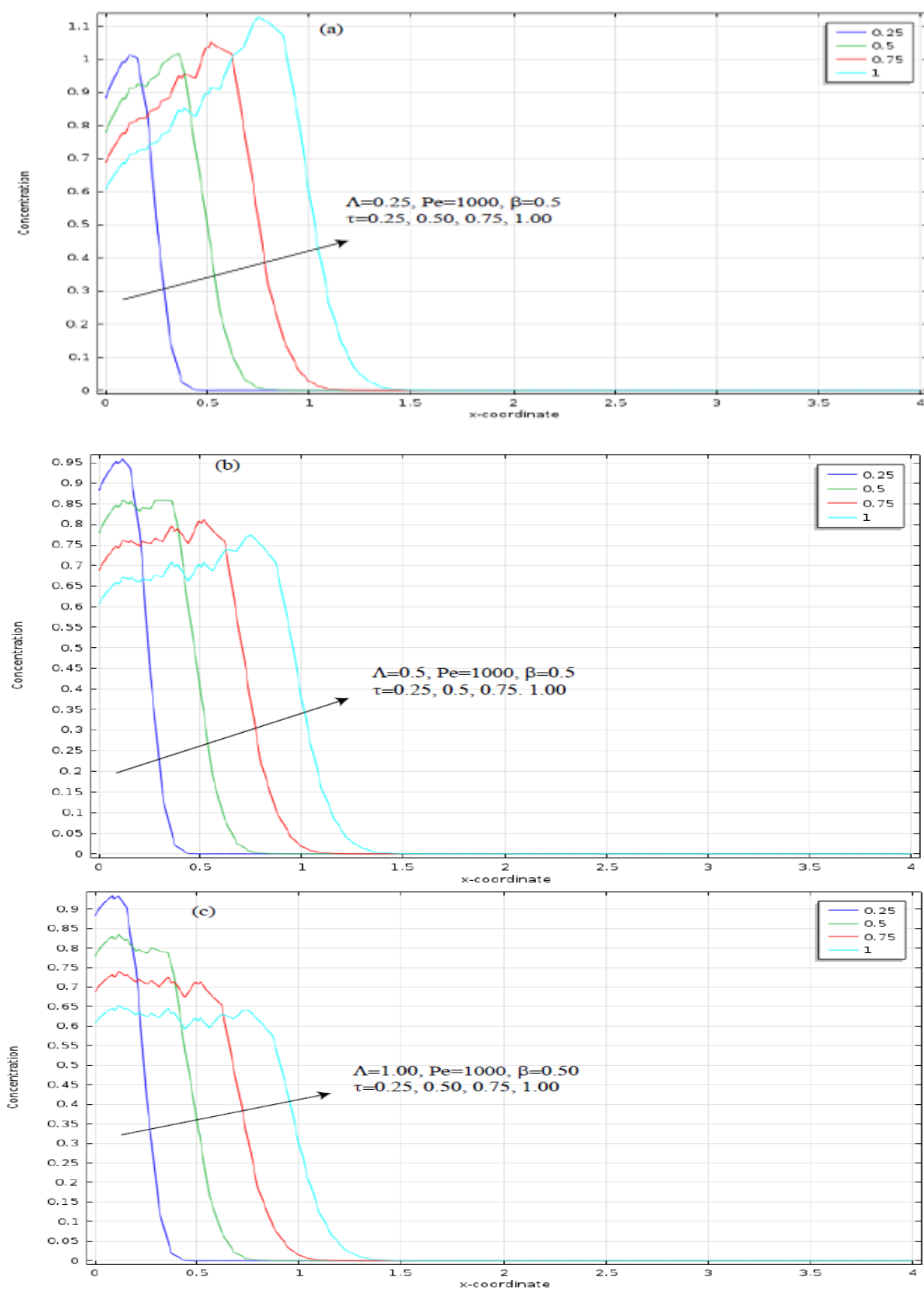
FIGURE 5: EXPONENTIAL SOURCE LINE GRAPHS FOR CONCENTRATION VS. LONGITUDINAL DISTANCE
