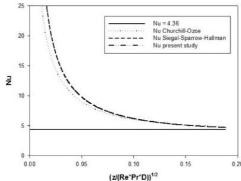
FIGURE 3. GRID VALIDATION BY MEANS OF CHURCHILL AND OZOE, SIEGAL-SPARROW-HALLMAN
