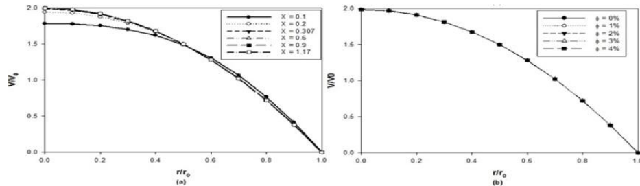
FIGURE 2. (a) PROFILES OF AXIAL VELOCITY AT SEVERAL LOCATIONS FOR Re = 1050 , q = 5000 W/m^2 , \Phi = 4\% . (b) PROFILES OF AXIAL VELOCITY AT x = 0.307m for Re = 1050 , q = 5000 W/m^2 AND SEVERAL VOLUME FRACTIONS.
