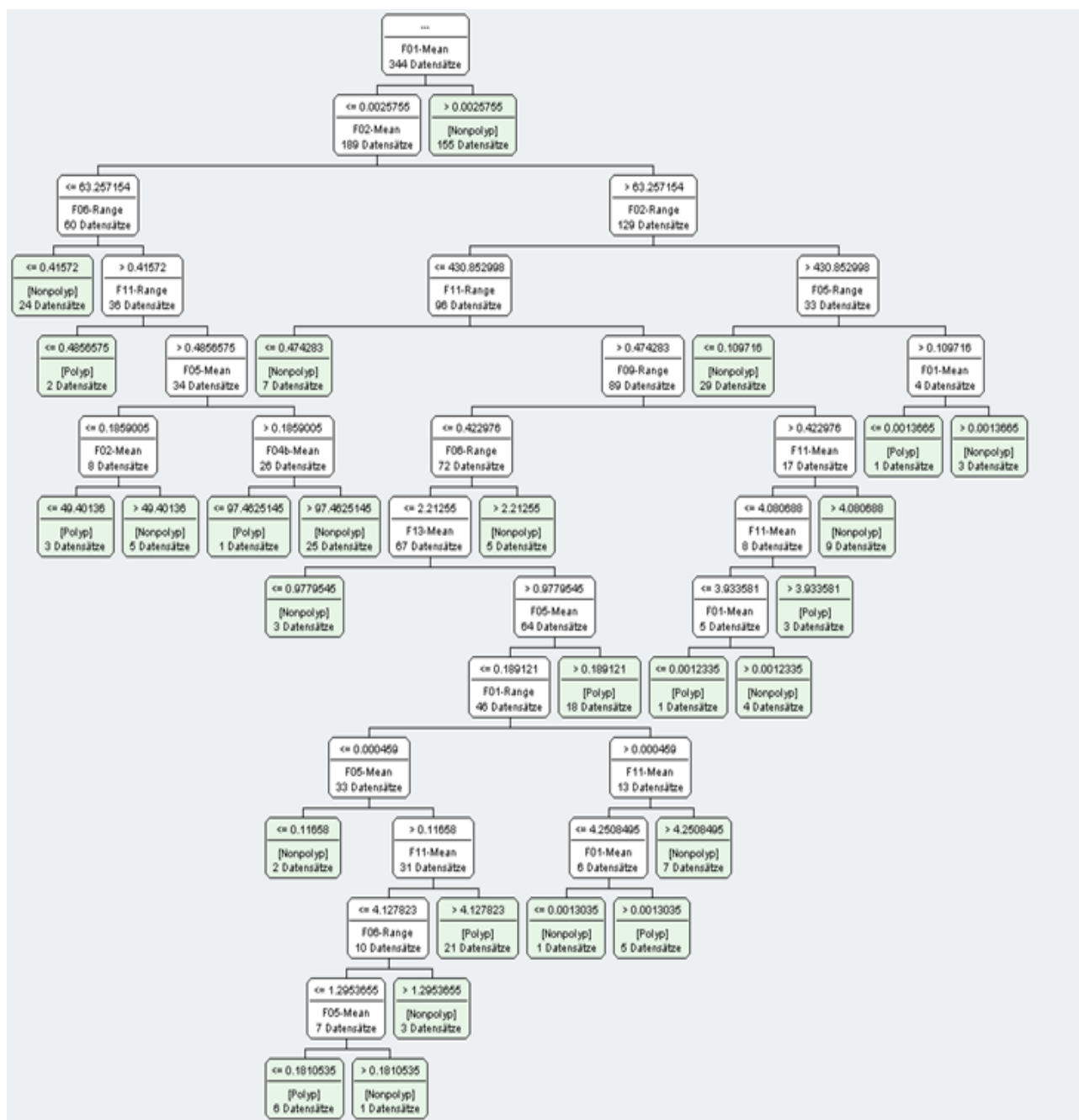
FIG. 5. DECISION TREE FOR COO FEATURE DESCRIPTOR
