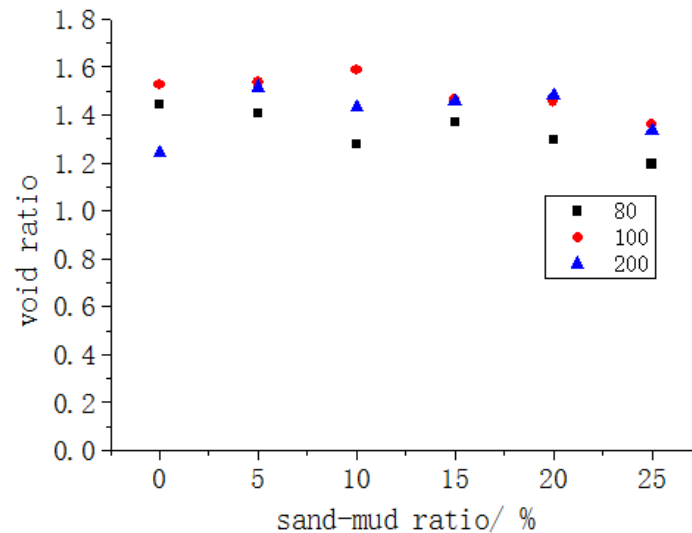
FIG. 12 RELATIONSHIP BETWEEN VOID RATIO AND SAND-MUD RATIO
