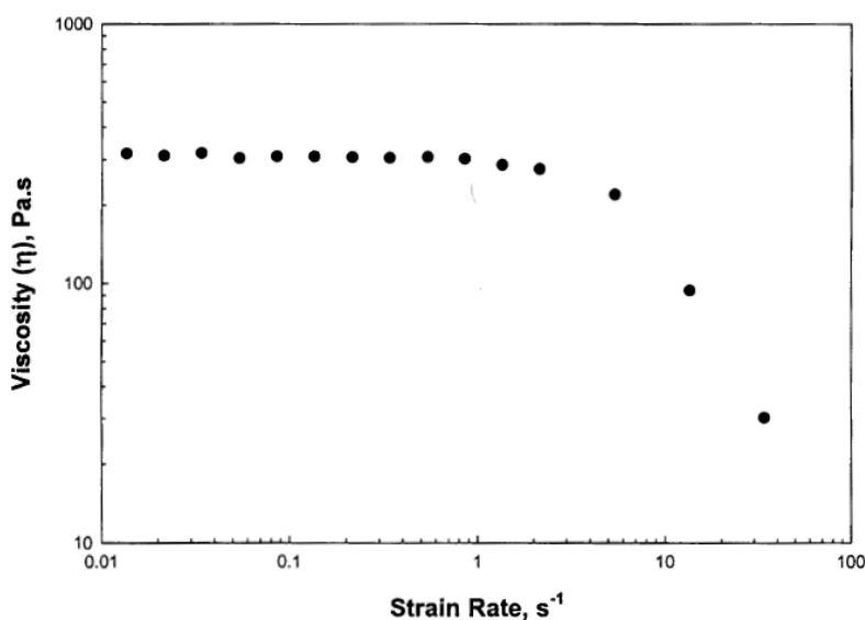
FIGURE 2. STEADY-STATE SIMPLE SHEAR VISCOSITY OF PDMS AS A FUNCTION OF SHEAR RATE USING A WEISSENBERG RHEOGONIOMETER.
