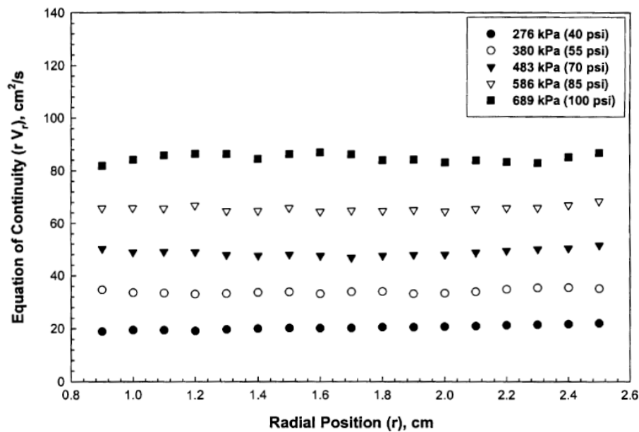
FIGURE 6. EQUATION OF CONTINUITY AS A FUNCTION OF THE CENTERLINE RADIAL POSITION FOR VARIOUS PRESSURE DROPS ACROSS THE FLOW CELL.
