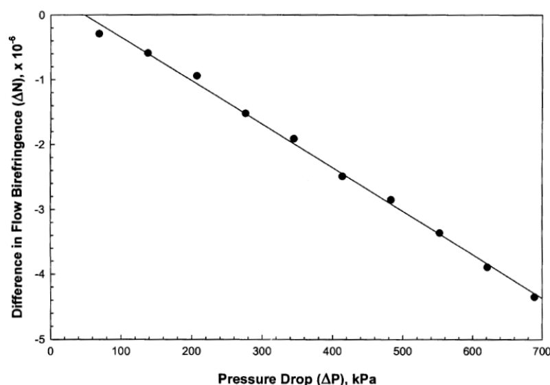
FIGURE 3. DIFFERENCE IN CENTERLINE BIREFRINGENCE (BETWEEN r = 1.1 cm AND r = 2.1 cm) AS A FUNCTION OF PRESSURE DROP ACROSS THE FLOW CELL.
