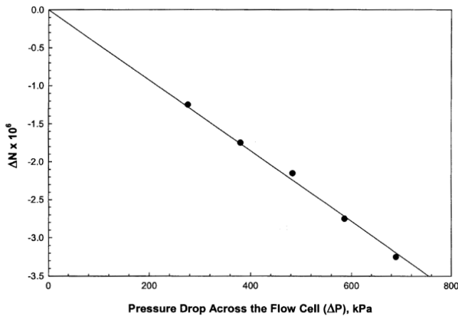
FIGURE 4. AVERAGE CENTERLINE BIREFRINGENCE AS A FUNCTION OF PRESSURE DROPS ACROSS THE FLOW CELL.
