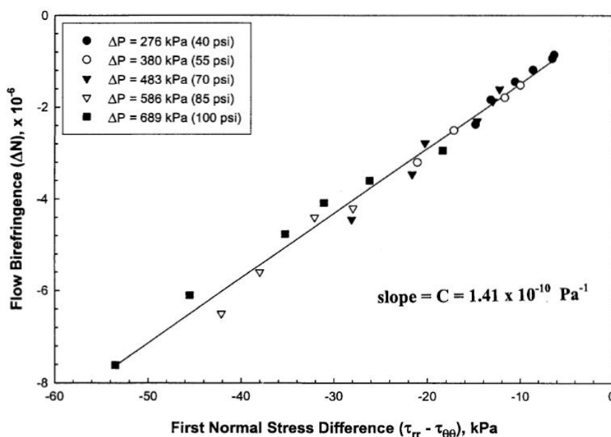
FIGURE 7. MEASURED FLOW BIREFRINGENCE VS. COMPUTED FIRST NORMAL STRESS DIFFERENCE (USING THE TWO-TERM GODDARD-MILLER MODEL) IN PLANAR EXTENSIONAL FLOW ALONG THE CELL CENTERLINE FOR VARIOUS PRESSURE DROPS ACROSS THE FLOW CELL.
