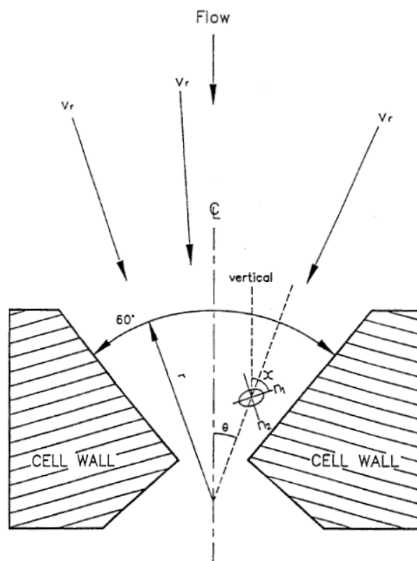
FIGURE 1. GEOMETRY OF THE TWO-DIMENSIONAL JEFFREY-HAMEL TYPE CONVERGING WEDGE FLOW CELL
