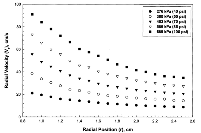
FIGURE 5. CENTERLINE RADIAL VELOCITY AS A FUNCTION OF RADIAL POSITION FOR VARIOUS PRESSURE DROPS ACROSS THE FLOW CELL.
