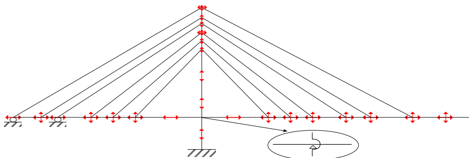
FIGURE 12 ADDITIONAL GEOMETRIC CONSTRAINTS IN THE G.TCUD METHOD FOR A HALF MODEL OF A CABLE-STAYED BRIDGE HAVING ONE INTERMEDIATE PIER
