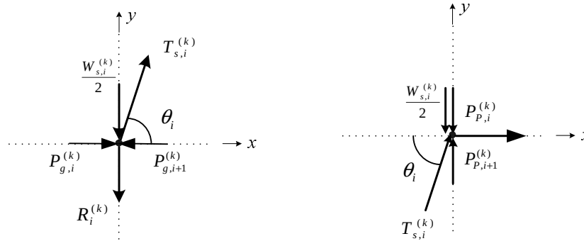
FIGURE 5 FREE BODY DIAGRAMS AT TWO ANCHORAGE POINTS OF ONE STAY CABLE
