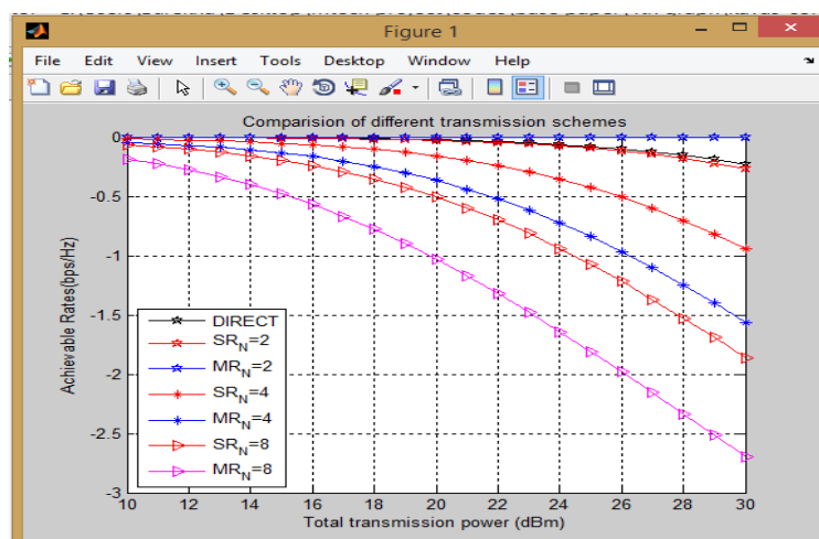
FIG.4 COMPARISION OF DIFFERENT TRANSMISSION SCHEMES
