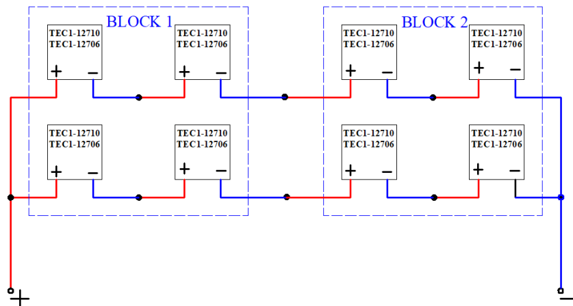
FIGURE 5. PARALLEL CONNECTION IMAGE OF 4 SERIAL SERIES OF TWO GROUPS TEC1-12706 AND TEC1-12710 THERMOELECTRIC MODULES
