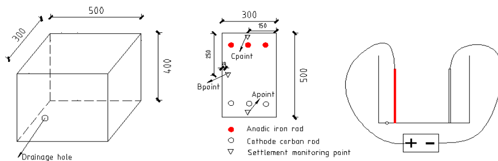
FIGURE 1: EXPERIMENTAL LAYOUT
