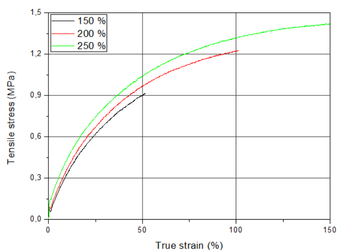
FIG. 3: RESULTS OF TENSILE TEST OF PDLLA FOIL IN CASE OF DIFFERENT DEFORMATION RANGE
