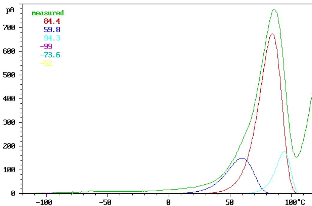
FIG. 7: TSD CURVES OF PLLA FOIL (5K/MIN↓; 5K/MIN ↑)
