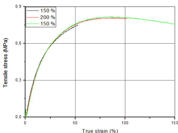
FIG. 2: RESULTS OF TENSILE TEST OF PET FOIL INN CASE OF DIFFERENT DEFORMATION RANGE
