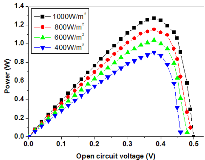
FIGURE 5. P-V CURVES FOR DIFFERENT SOLAR RADIATIONS
