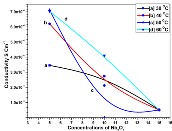
FIGURE.4: CONDUCTIVITY VARIATION WITH (POLYMER/SALT) WITH VARYING \text{Nb}_2\text{O}_5 CONCENTRATION AT DIFFERENT TEMPERATURES.
