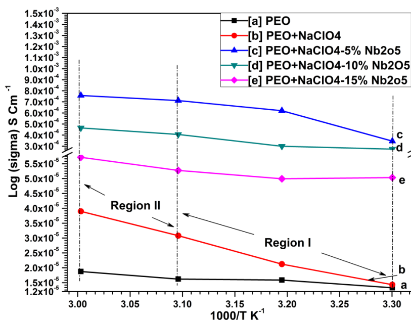
FIGURE.3: Arrhenius type Temperature dependent conductivity plots of [a]PEO, [b]PEO:NaClO 4 ::25:1, [c]PEO-NaClO 4 -5 Wt.% Nb 2 O 5 ; [d]PEO-NaClO 4 -10 wt.% Nb 2 O 5 ; [e]PEO-NaClO 4 -5 Wt.% Nb 2 O 5 -15 wt.% Nb 2 O 5 .
