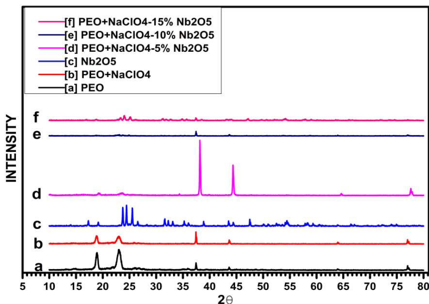
FIGURE 1: [a] PEO, [b] PEO-NaClO 4 , [c]Nb 2 O 5 , [d]PEO-NaClO 4 -5Wt.% Nb 2 O 5 , [e]PEO-NaClO 4 10Wt.% Nb 2 O 5 ,[f] PEO-NaClO 4 -15 Wt.%Nb 2 O 5 .
