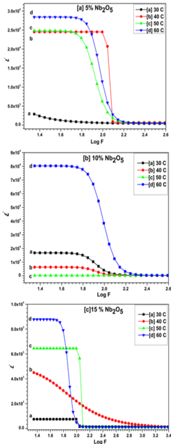
FIGURE.6.[A],[B]&[C] VARIATION OF DIELECTRIC CONSTANT ( \epsilon' ) WITH RESPECT TO FREQUENCY AT VARIOUS TEMPERATURES OF 5, 10, 15Wt.% \text{Nb}_2\text{O}_5 RESPECTIVELY
