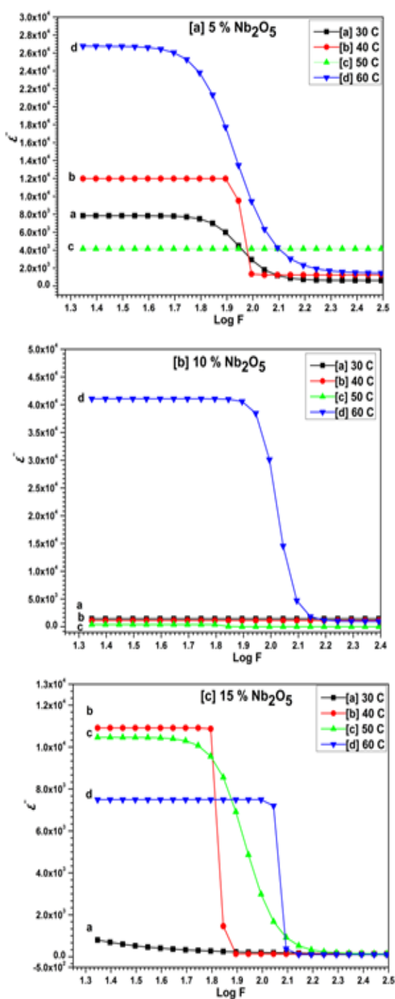
FIGURE.7. [A],[B]&[C] VARIATION OF DIELECTRIC LOSS ( \epsilon'' ) WITH RESPECT TO FREQUENCY AT VARIOUS TEMPERATURES OF 5, 10, 15Wt.% \text{Nb}_2\text{O}_5 RESPECTIVELY.
