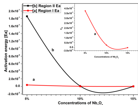
FIGURE.5: VARIATION OF ACTIVATION ENERGY ( E_a ) WITH DIFFER CONCENTRATIONS OF (A) ABOVE THE MELTING TEMPERATURE. (B) BELOW THE MELTING TEMPERATURE WITH \text{Nb}_2\text{O}_5 CONCENTRATION
