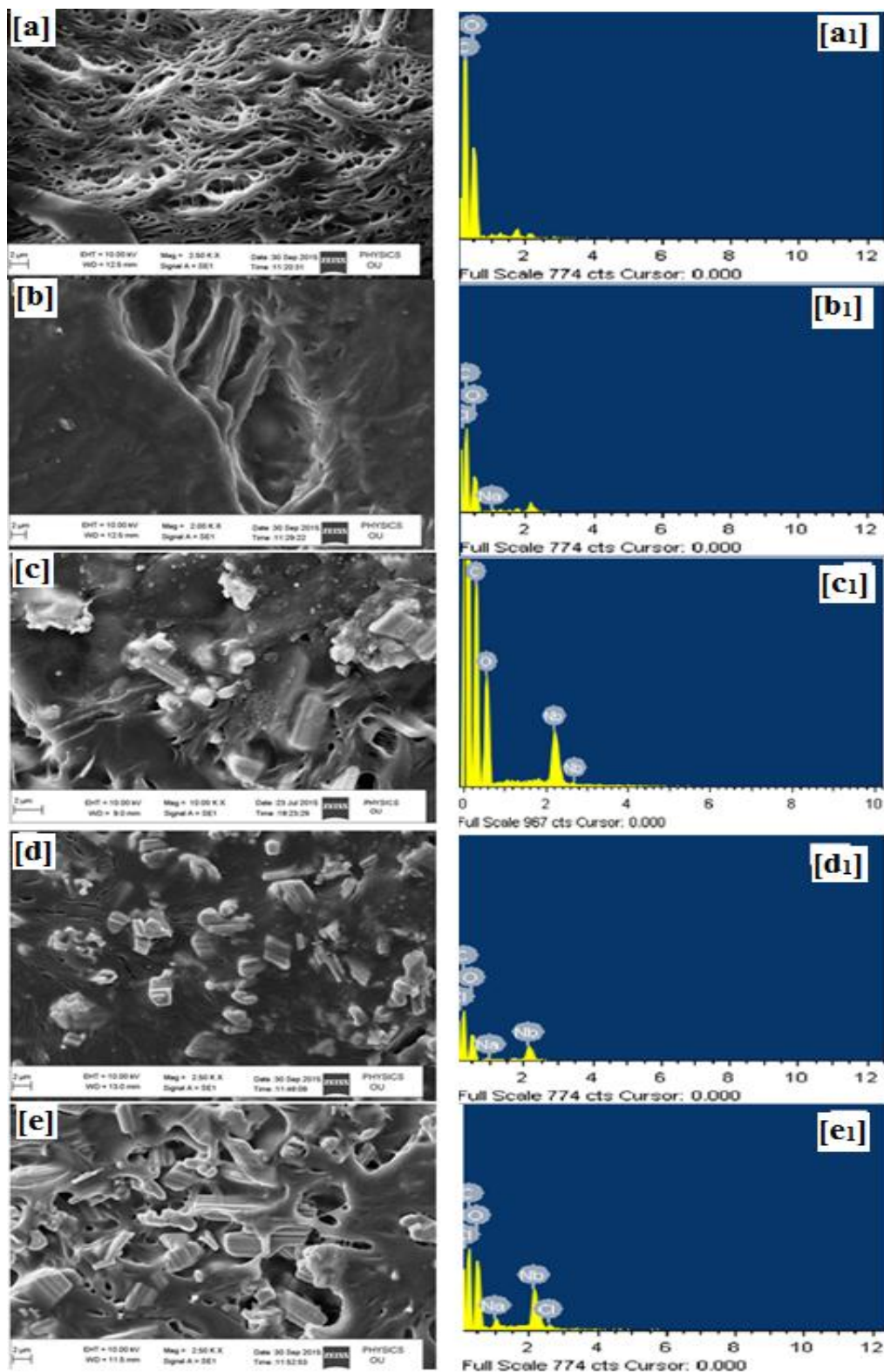
FIGURE.2: SEM Images [a]PEO, [b]PEO-NaClO 4 , [c]Nb 2 O 5 ,[d]PEO-NaClO 4 -5Wt.%Nb 2 O 5 , [e]PEO-NaClO 4 -10Wt.%Nb 2 O 5 ,[f]PEO-NaClO 4 -15 Wt.% Nb 2 O 5 , and EDAX images[a1]PEO,[b1]PEO-NaClO 4 ,[c1]Nb 2 O 5 ,[d1]PEO-NaClO 4 -5Wt.%Nb 2 O 5 ,[e1]PEO-NaClO 4 -10Wt.%Nb 2 O 5 ,[f1]PEO-NaClO 4 -15 Wt.% Nb 2 O 5 .
