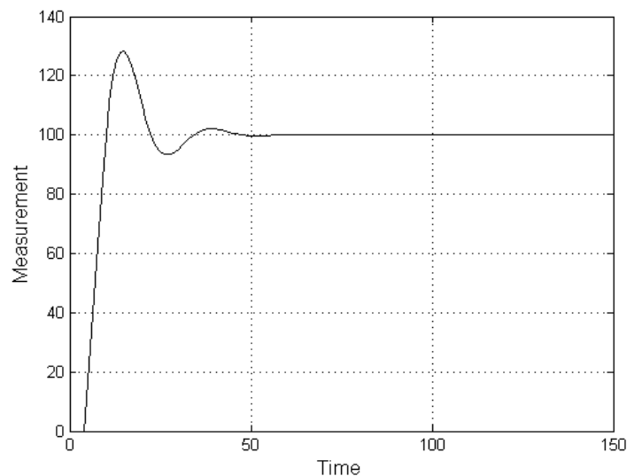
FIG. 2 PROFESSIONAL PID
