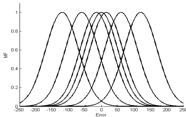
FIG. 2. MEMBERSHIP FUNCTION OF ERROR.
