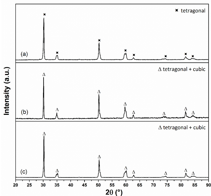
FIGURE 1. XRD PATTERNS OF (DY, CE)-YSZ: (A) 3DY5CE-YSZ; (B) 2DY-YSZ; (C) 4YSZ
