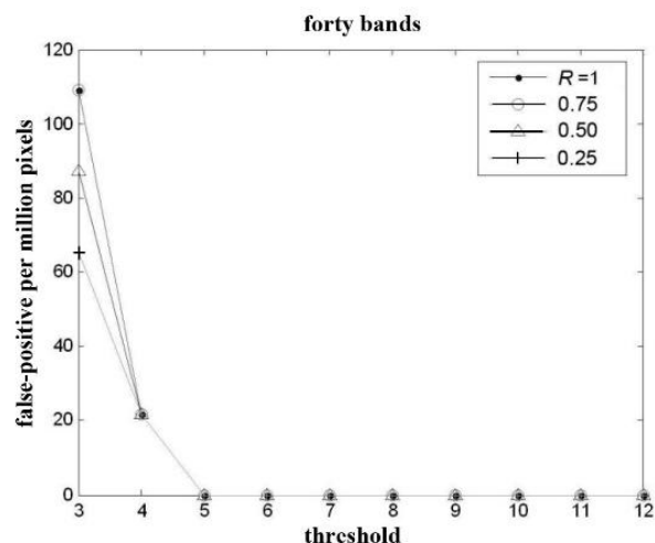
FIGURE 8. NUMBER OF FALSELY LABELED PIXELS PER ONE-MILLION INPUT PIXELS IS PLOTTED AS FUNCTION OF INCONGRUENCE-THRESHOLD H . BAND-THRESHOLD IS FIXED AT Q = 40 AND FALSE-ALARM PERFORMANCE IS PLOTTED FOR CONTAMINATION FACTOR (CF) OF R = 0.25, 0.5, 0.75 , AND 1 .
