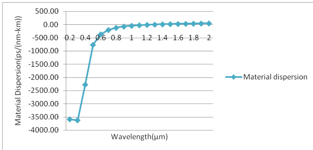
FIG. 3 MATERIAL DISPERSION OF FUSED SILICA GLASS
