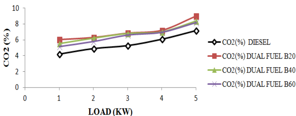
Fig. 7 Variations in CO 2 with change in load
