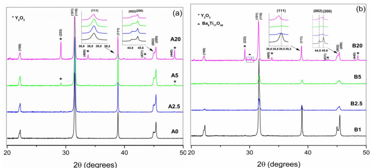
FIG. 2. X-ray diffraction patterns of undoped \text{BaTiO}_3 ( 1350^\circ\text{C} ) and \text{Y}_2\text{O}_3 - 2.5, 5 and 20 wt% - doped \text{BaTiO}_3 ( 1350^\circ\text{C} ) powder. Powder coming from (a) BT-A and (b) BT-B.
