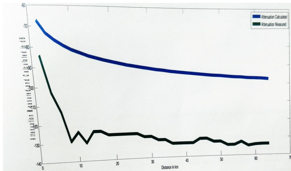
FIGURE 2: GRAPH OF ATTENUATION MEASURED AND ATTENUATION CALCULATED AGAINST DISTANCE
