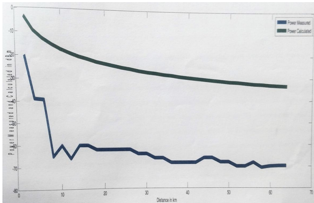
FIG 1: POWER MEASURED AND POWER RECEIVED AGAINST DISTANCE
