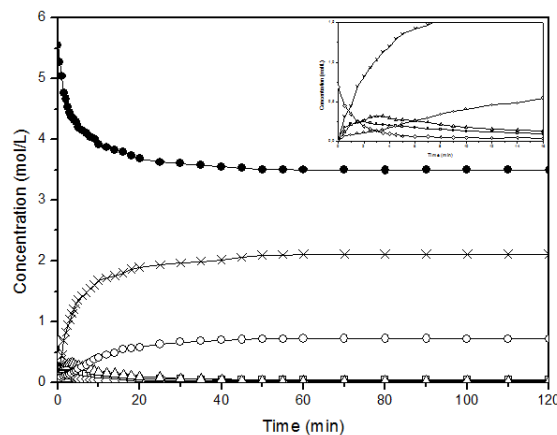
FIG. 1 –THE COMPOSITION OF THE REACTION MIXTURE DURING THE TRANSESTERIFICATION OF SOYBEAN OIL AT 308.15 K. EXPERIMENTAL DATA: (—◇—) TRIACYLGLYCEROL; (—□—) DIACYLGLYCEROL; (—Δ—) MONOACYLGLYCEROL; (—×—) ETHYL ESTER; (—○—) GLYCEROL AND (—●—) ETHANOL.
