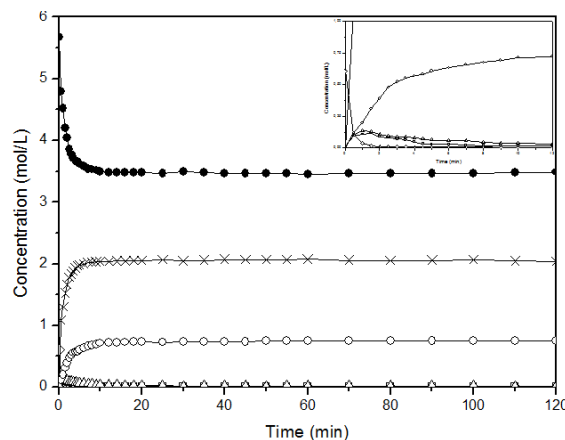
FIG. 2 – THE COMPOSITION OF THE REACTION MIXTURE DURING THE TRANSESTERIFICATION OF SUNFLOWER OIL AT 338.15 K. EXPERIMENTAL DATA: (—◇—) TRIACYLGLYCEROL; (—□—) DIACYLGLYCEROL; (—Δ—) MONOACYLGLYCEROL; (—×—) ETHYL ESTER; (—○—) GLYCEROL AND (—●—) ETHANOL.
