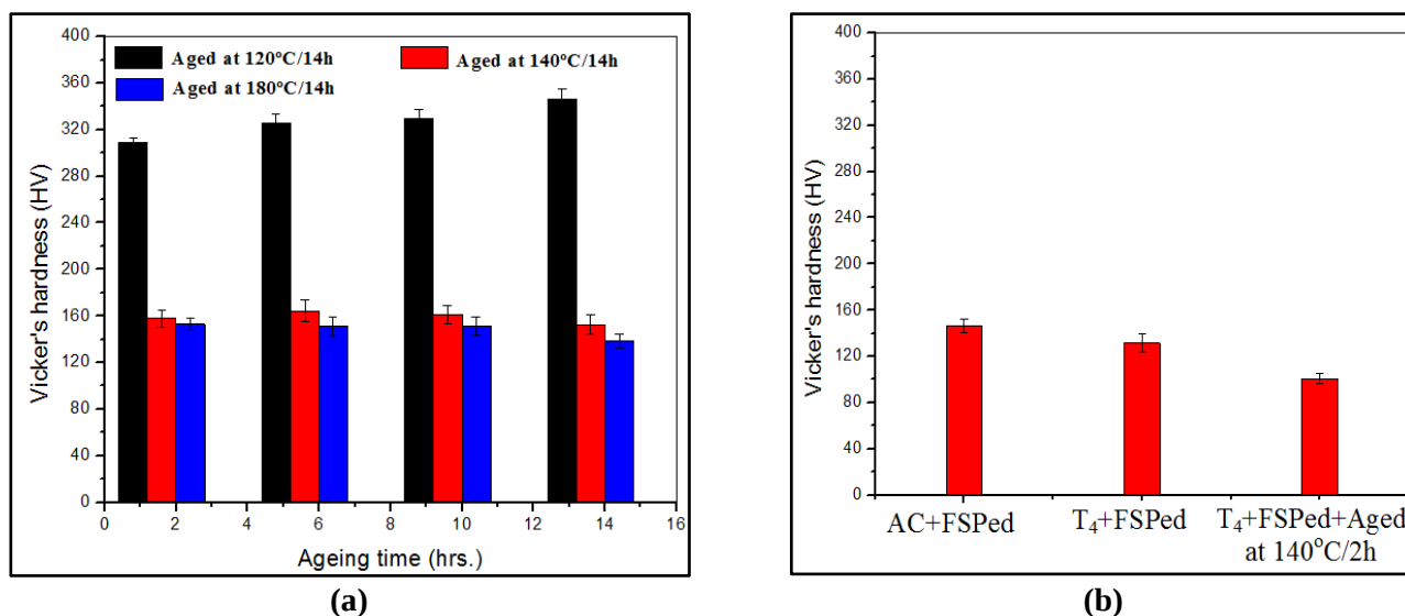
FIGURE 8: The Vicker's hardness bar diagrams are exhibited hardening effect at different conditions: (a) after different ageing treatments, and (b) after different FSPed conditions. (1000 rpm and 70 mm/min)
