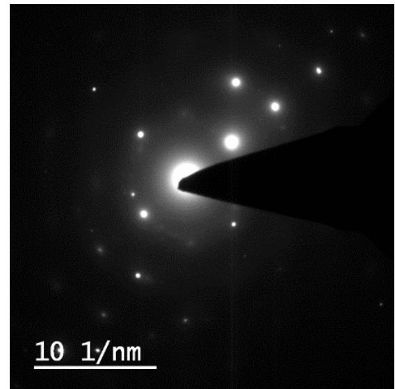
FIGURE 6: TEM micrographs with SAD patterns of 7075 Al alloy ( T_4 +FSP+Post-aged at 140^\circ\text{C} for 2h): (a) at low magnification (500 nm), (b) at high magnification (200 nm). (1000 rpm and 70 mm/min).
