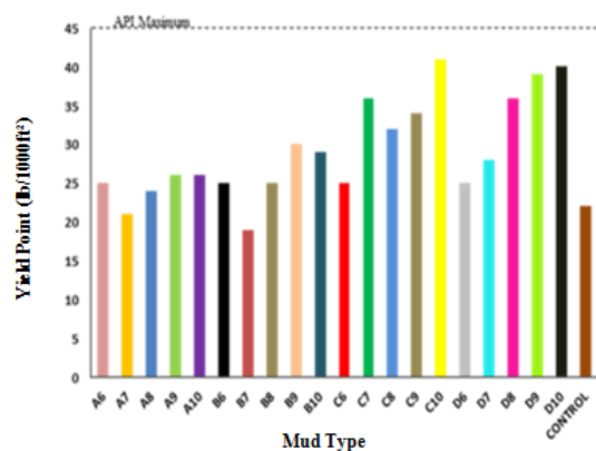
FIGURE 5: Yield Point for TMS98/0581 starch-bentonite formulated muds
