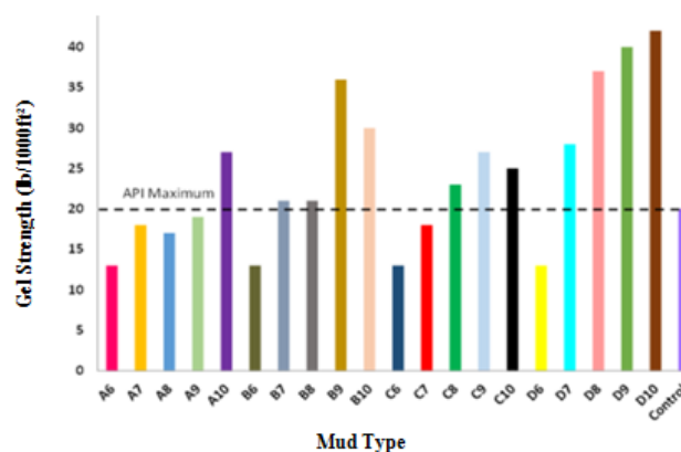
FIGURE 8: 10 Secs Gel Strength for TMS 98/0581 Starch-Bentonite formulated muds
