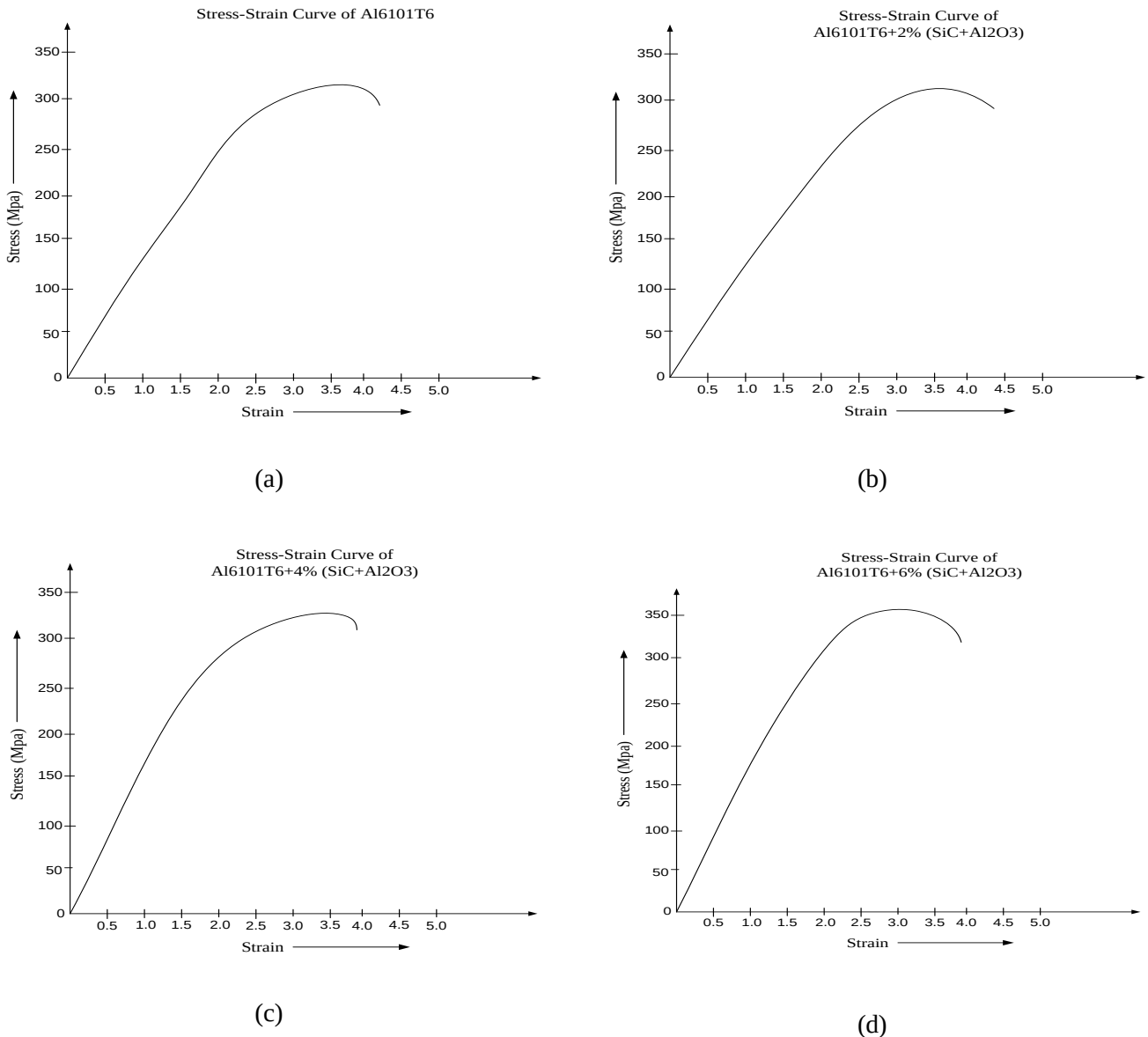
FIGURE 6: Stress Strain Curve for (a) Al 6101 T6 (b) 2% SiC and \text{Al}_2\text{O}_3 (c) 4% SiC and \text{Al}_2\text{O}_3 (d) 6 % SiC and \text{Al}_2\text{O}_3
