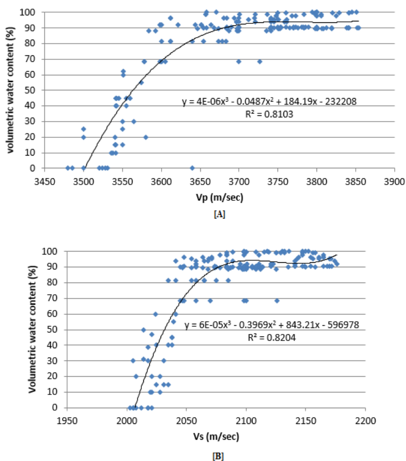
FIG. 3: PIETRA GENTILE: ULTRASONIC WAVE VELOCITY VS VOLUMETRIC WATER CONTENT: A) P-WAVE; B) S- WAVE
