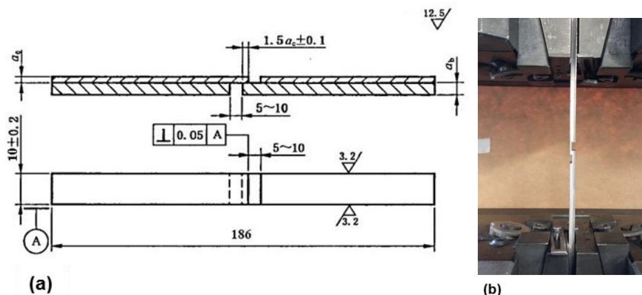
Fig. 6: Tensile shear test sample (a) schematically and (b) during testing
