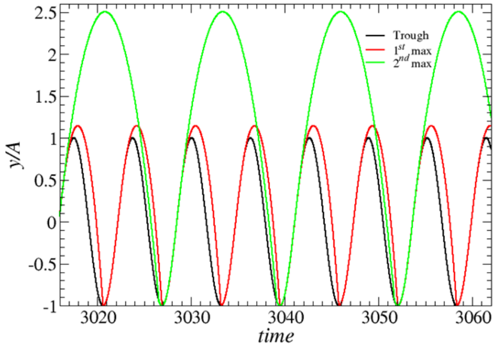
FIG. 5: The vertical motion of the table (black solid line) and of the granular block at the first maximum \Gamma=1.7 (red solid lined) and the second maximum \Gamma=4.8 (green solid line) as function of time, calculated using a solid friction coefficient \mu = 0.3 .
