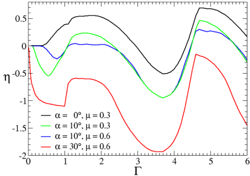
FIG. 2: The transport velocity efficiency \eta = hv/A\omega i as function of the throw number \Gamma = A\omega^2/g\cos(\alpha) calculated using \varepsilon_t = 0.7 and \mu = 0.3 for \alpha = 0^\circ (black) and \alpha = 10^\circ (green). The velocity efficiency (in blue and red) is calculated using the same tangential restitution coefficient \varepsilon_t = 0.7 while the friction coefficient was set to \mu = 0.6 for \alpha = 10^\circ and \alpha = 30^\circ respectively.
