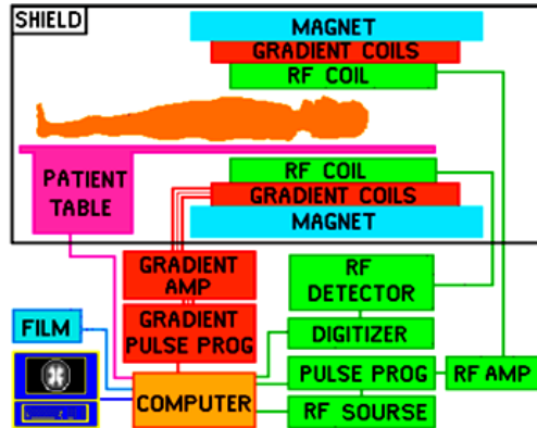
FIGURE 1: ENLARGED VIEW OF MRI SYSTEM
