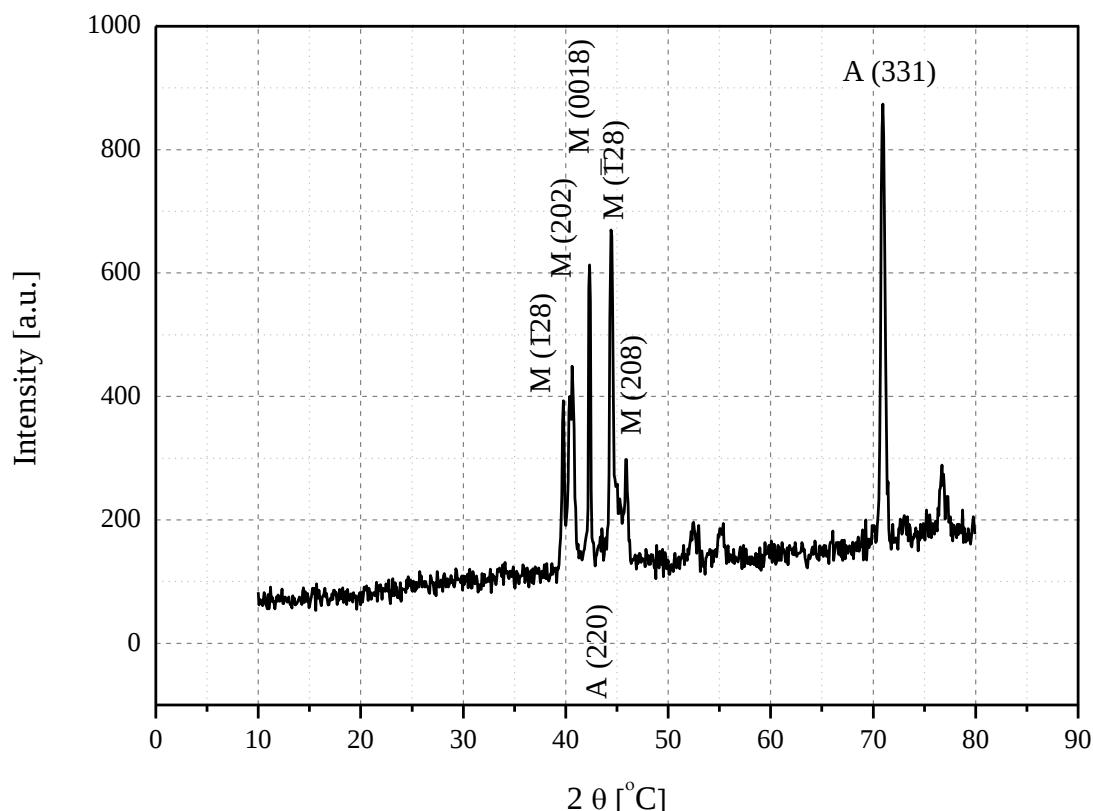
FIGURE 12. X-RAY DIFFRACTOGRAM OF THE QUENCHED ALLOY
