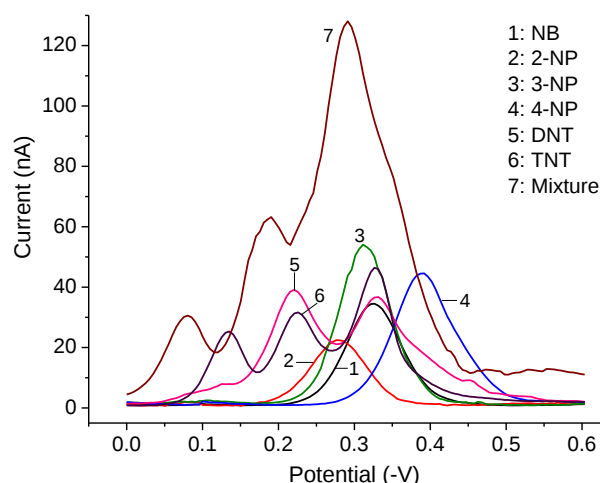
FIG 1: THE VOLTAMMOGRAMS OF NB, 2-NP, 3-NP, 4-NP, DNT, TNT (1PPM) AND THEIR MIXTURES
