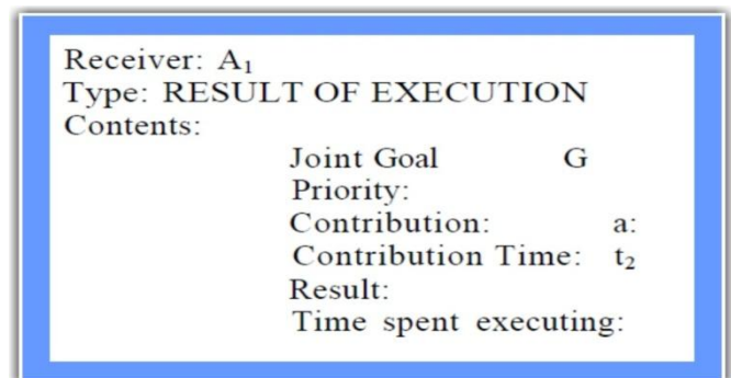
FIGURE 7: Execution result
