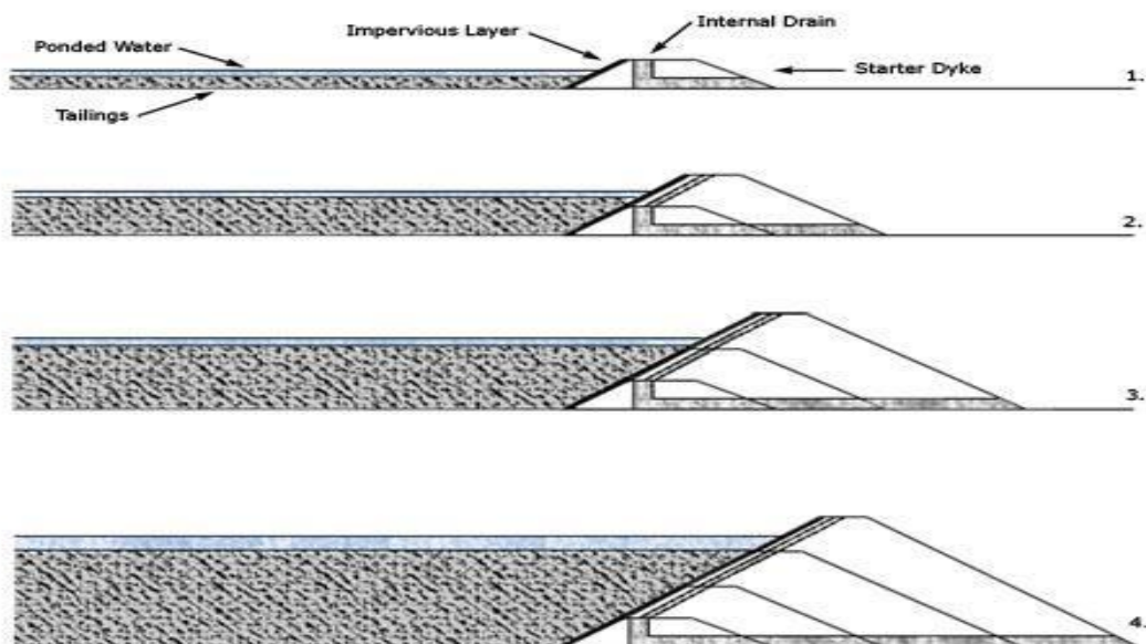
FIGURE: (II) DOWN-STREAM CONSTRUCTION METHOD
