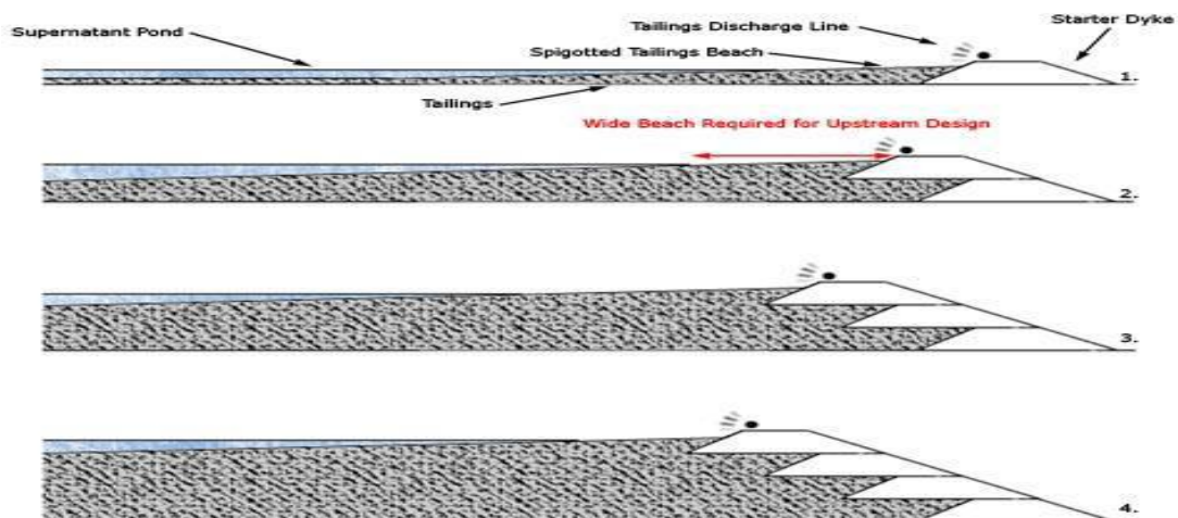
FIGURE (I) UP-STREAM CONSTRUCTION METHOD.
