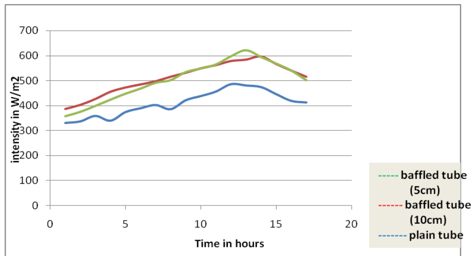
FIG. 2 GRAPH BETWEEN TIME AND INTENSITY
