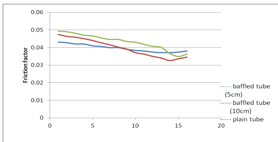
FIG.- 5 GRAPH BETWEEN TIME AND FRICTION FACTOR
