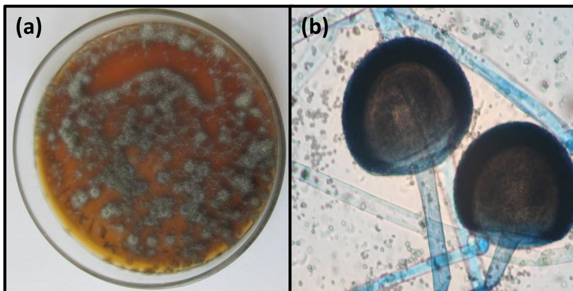
FIGURE 2. COLONY MORPHOLOGY AND MICROSCOPICAL OBSERVATION OF R.ORYZAE
