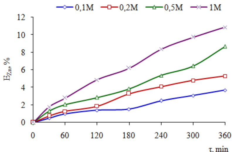
FIG. 3 EXTRACTION DEGREE OF ZINC DURING ELEKTROLEACHING THE CONCENTRATE, DEPENDING ON THE CONCENTRATION OF SODIUM HYDROXIDE
