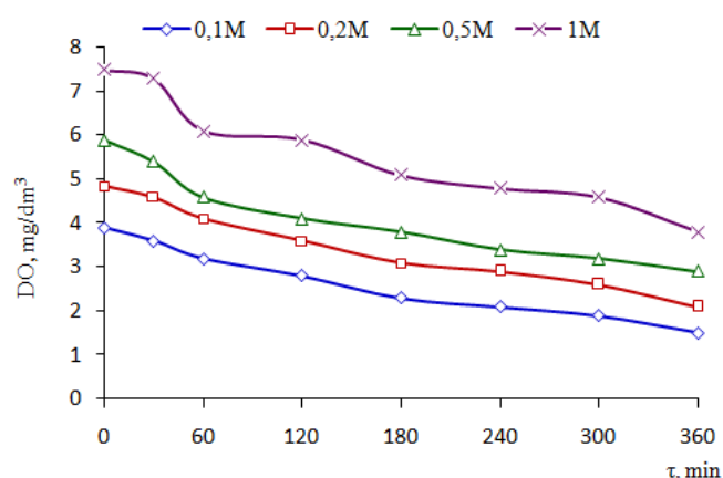
FIG. 5 THE CHANGE IN THE OXYGEN CONCENTRATION OF SOLUTIONS DURING LEACHING PROCESS OF THE CONCENTRATE, DEPENDING OF THE CONCENTRATION
