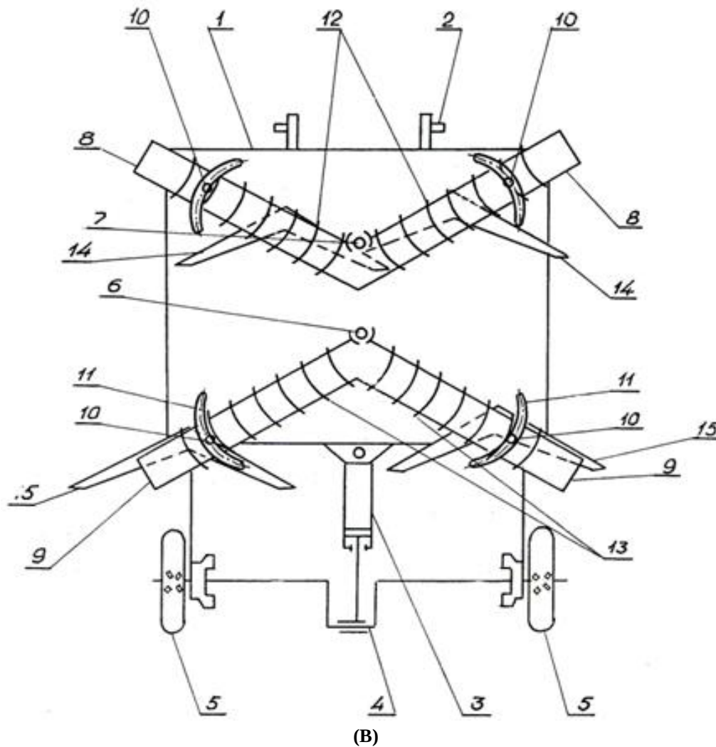
FIGURE 1: STRUCTURAL LAYOUT
